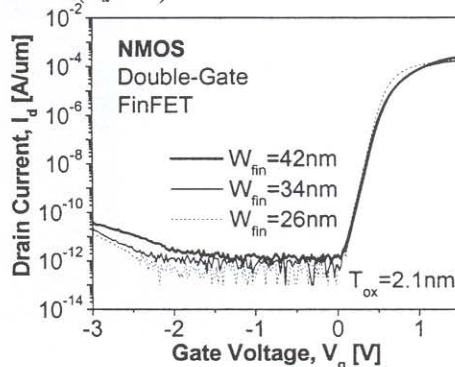
Fig. 6 Measured I_d - V_g characteristics of symmetrical DG-FinFET. A thinner body gives lower GIDL current
