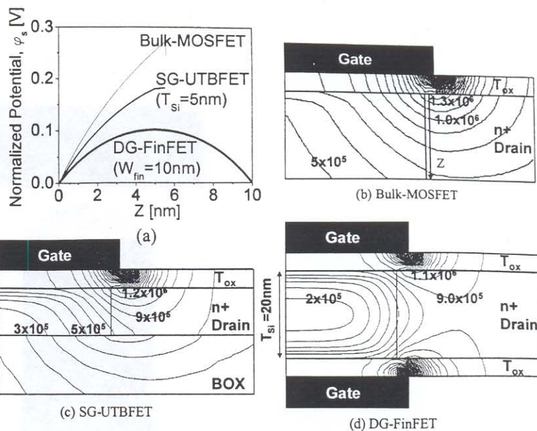
Fig. 2 Potential profile (a) and 2-D electric field profile (b)-(d) for bulk-MOSFET, SG-UTBFET, and DG-FinFET ( V_g=-1V , V_d=1V , T_{ox}=2.0nm , N+=1.0 \times 10^{18} cm^{-3} ).
